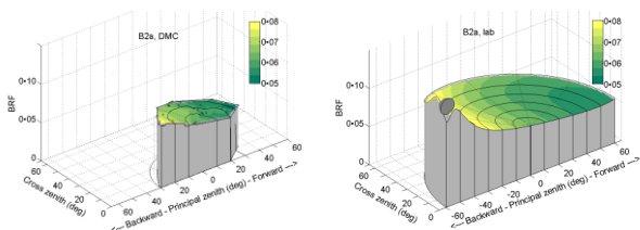
Figure 4. 3D-BRF plot of black gravel measured by the DMC (left) and at laboratory (right). (Honkavaara et al., 2011)
