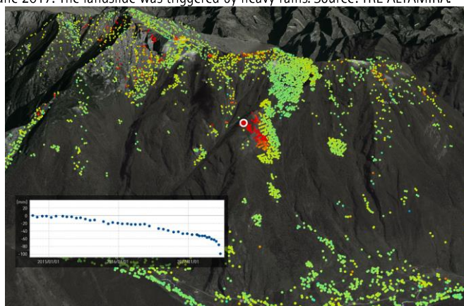
Figure 1: InSAR time series analysis of precursory of the landslide that hit a village in Maoxian county in Sichuan province, China in June 2017. The landslide was triggered by heavy rains. Source: TRE ALTAMIRA.
