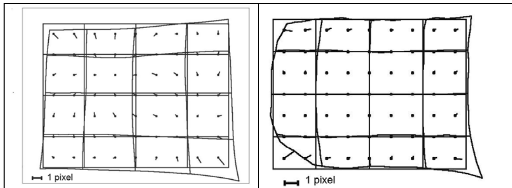
Fig. 3: Systematic image errors of a digital mid-format (36.8mm x 49.2mm, 6.8µm pixel size) and a digital small-format (5.7mm x 4.3mm, 1.8µm pixel size) camera (not Z/I Imaging and Vexcel Imaging) after eliminating the effect of radial symmetric distortion.
