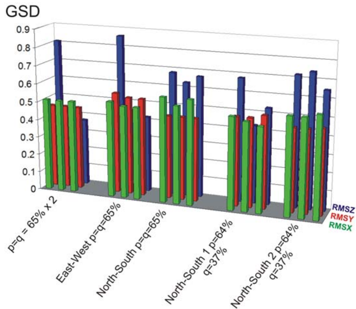
Fig. 9: Bundle block adjustments with 5.7cm GSD, root mean square differences at check points, left columns: without additional parameters, center column: additional parameters 1 – 12, right hand column: additional parameters 1 – 12 + 81 – 88. Whole block with 144 images, with p=q=65% 72 images, with q=37% 36 images.
