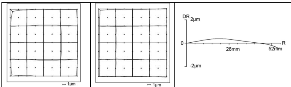
Fig. 5: Systematic image errors DMC II 140 with 9.5cm GSD left: whole effect, center: without radial symmetric distortion, right: radial symmetric lens distortion.
