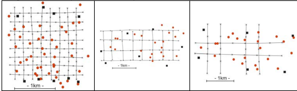
Fig. 1: Flight lines, control points (squares) and check points (red circles) of test flights; Left: 5.7cm GSD, center: 9.5cm GSD, right: 20.2cm GSD.
