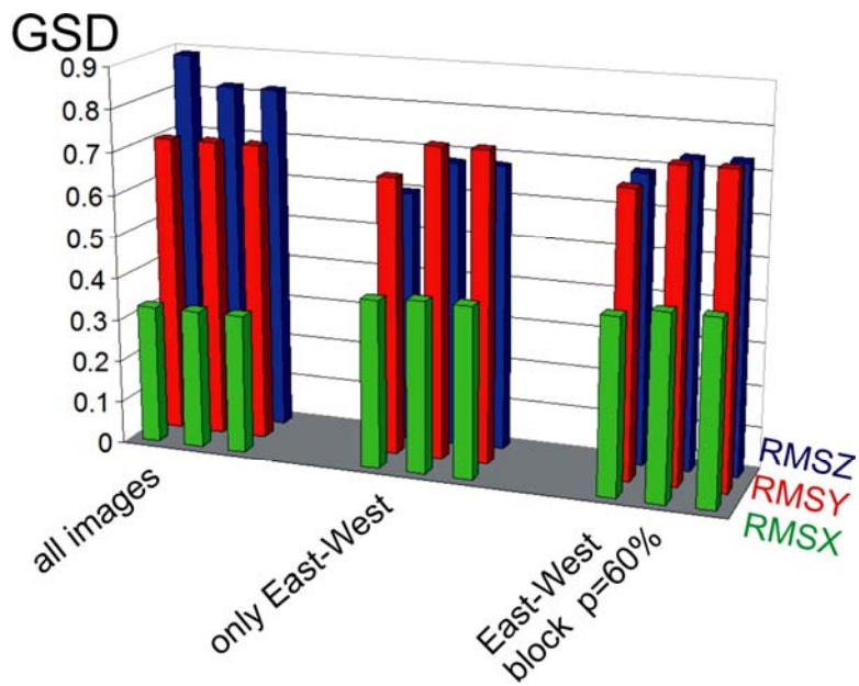
Fig. 11: Bundle block adjustments with 20.2cm GSD, root mean square differences at check points, left columns: without additional parameters, center column: additional parameters 1 – 12, right hand column: additional parameters 1 – 12 + 81 – 88. Whole block with 36 images, only East–West 18 images, only East–West with p=60\% 9 images.
