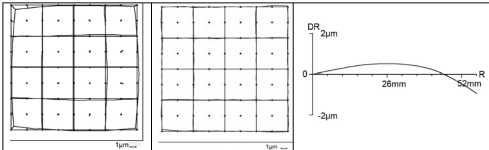
Fig. 4: Systematic image errors DMC II 140 with 5.7cm GSD left: whole effect, center: without radial symmetric distortion, right: radial symmetric lens distortion.
