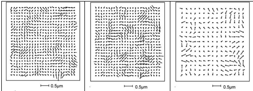
Fig. 7: Remaining systematic image errors of bundle block adjustments with self calibration by 12 additional parameters; left: related to 5.7cm GSD; center 9.5cm GSD; right: 20.2cm GSD.
