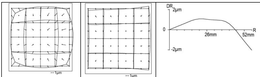
Fig. 6: Systematic image errors DMC II 140 with 20.2cm GSD left: whole effect, center: without radial symmetric distortion, right: radial symmetric lens distortion.
