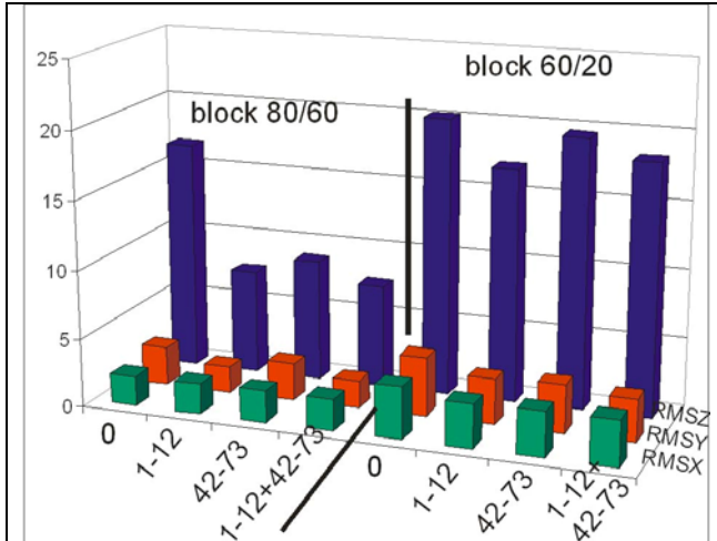
Figure 13: root mean square differences at check points
