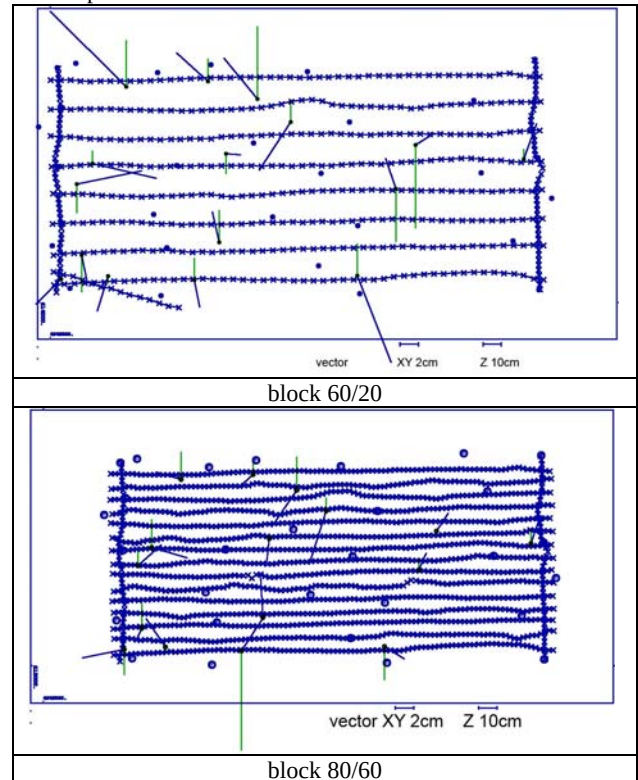
Figure 14: discrepancies at check points of block adjustment without self calibration green (vertical vector) = Z-discrepancies
