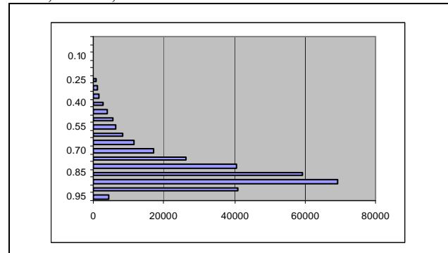
Figure 6: frequency distribution of least squares matching correlation coefficients – sub-area of Cartosat-1 Istranca vertical axis: correlation coefficient horizontal axis: number of matched points
