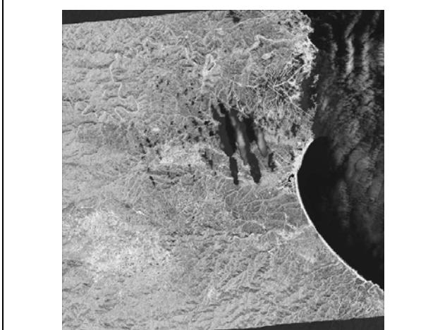
Figure 5: quality image - overlay to image with grey value depending upon correlation coefficient correlation coefficient r=1.0 = grey value 255 (white) r=0.5 = grey value 123 (grey)
