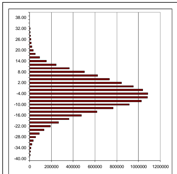
Figure 11: frequency distribution of height differences Cartosat-1 DSM against DEM25000
