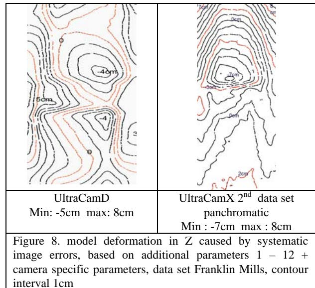
Figure 8. model deformation in Z caused by systematic image errors, based on additional parameters 1 – 12 + camera specific parameters, data set Franklin Mills, contour interval 1cm The figures 8 shows the model deformation of the Z-component caused by not respected additional parameters for the data set Franklin Mills. For the DMC it is between -1.5cm up to 2 cm, and for the RC30 between -4cm up to 3cm. The model deformation has been computed in the object space for a specific model and rotated to the base direction. Based on 0.5 pixels standard deviation of the x-parallax in a photogrammetric model, the expectation for the vertical accuracy for the DMC is 8.6cm, for the UltraCamX 6.8cm, for the UltraCamD 7.8cm and for the RC30 4cm. The varying values are depending upon the GSD and the height to base relation which is 3.1 for the DMC, 3.7 for the UltraCam and 1.6 for the wide angle RC30. The estimated standard deviations are not identical to the results of
