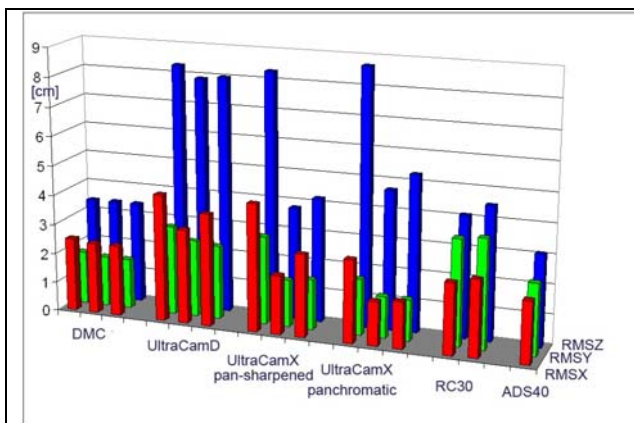
Figure 7. comparison of results at independent check points of block adjustments with 8 control points achieved in test area Franklin Mills based [cm] Within the groups: from left without self calibration / with parameters 1 – 12 / with parameters 1 – 12 + camera specific parameters
