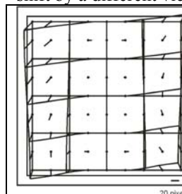
Fig. 4: image geometry determined by IRS-1C-calibration
