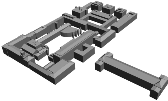
Figure 2: CAD-model of buildings (test area TUM)
