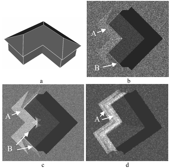
Figure 1: Simple building and SAR simulation. a) Model, b) SE-RAY-EM, c) FGAN-FOM, d) SARViz
