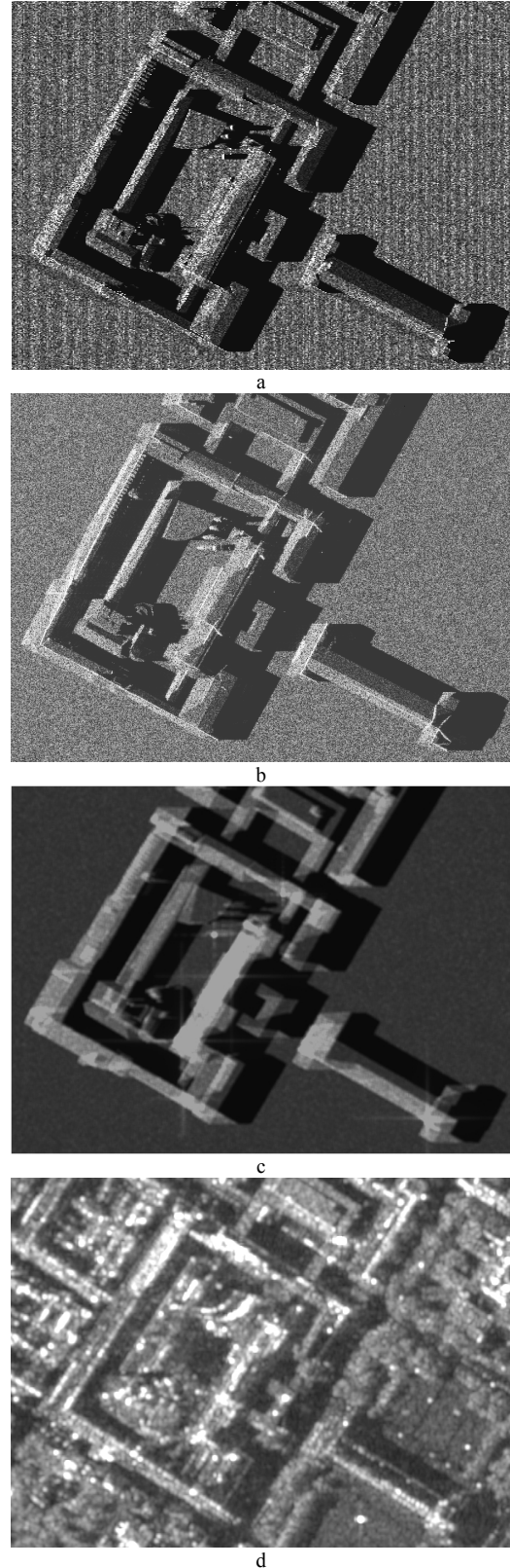
Figure 3: SAR simulation of buildings (test area TUM). a) SE-RAY-EM, b) FGAN-FOM, c) SAR Viz, d) SAR image (ESAR, DLR-HR)
