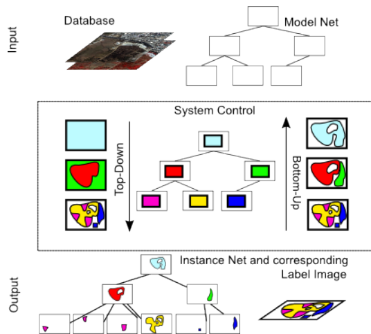
Figure 1: GEOAIDA Design
