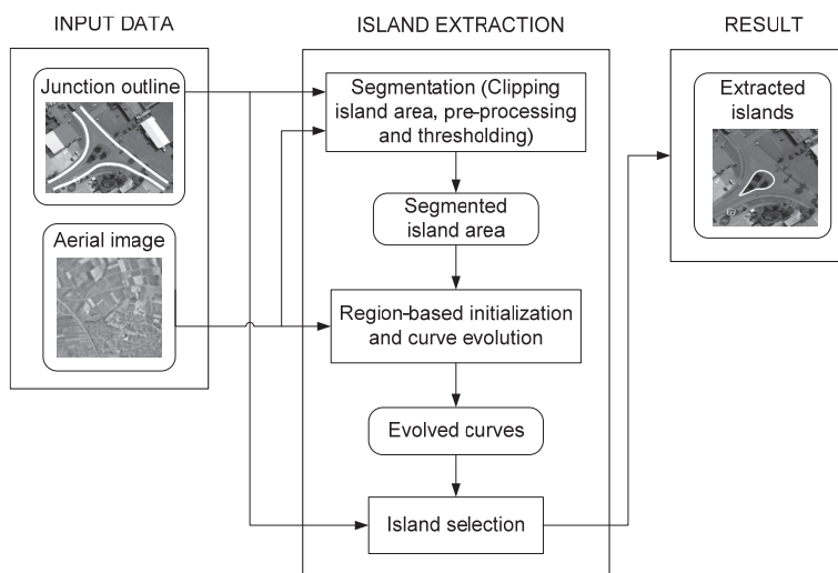
Fig. 4: Workflow of island extraction.
