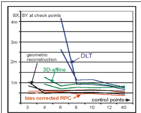
Fig. 10: orientation of QuickBird, Zonguldak (mountainous); root mean square discrepancies at independent check points as function of GCP number - 40 GCPs = discrepancies at GCPs
