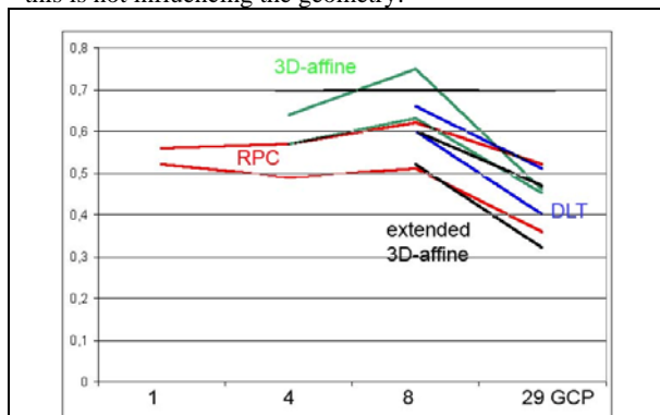
Fig. 9: accuracy of point determination by WorldView-1, Istanbul, depending upon number of control points; upper line = standard deviation in view direction, lower line across
