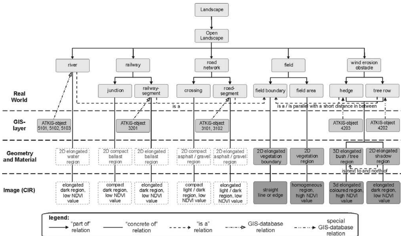
Figure 1. Semantic Model
