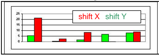
Figure 10: shift values for X and Y for Geo-images corrected by DEM [m] (projects Switzerland, USA, Malaysia, 2 x Turkey)
