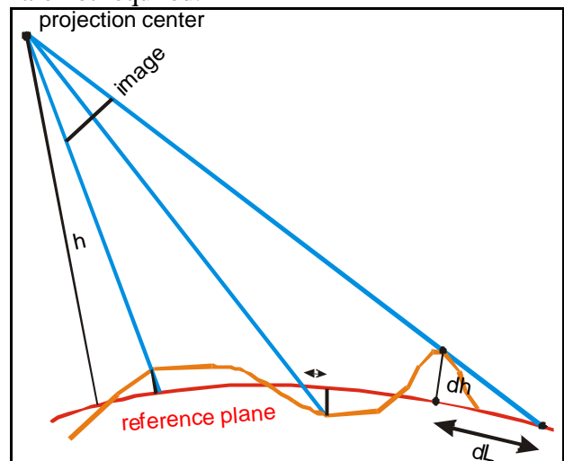
Figure 9: geometric situation of CARTERRA-Geo-images (rectified IKONOS-images)
