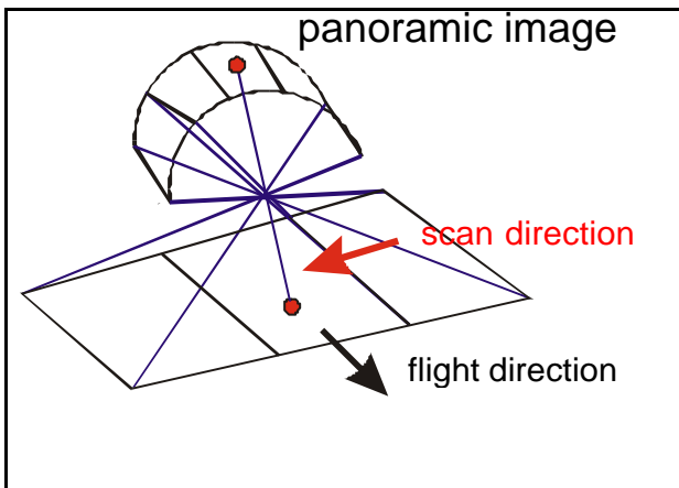
Figure 3: geometric principal of panoramic cameras
