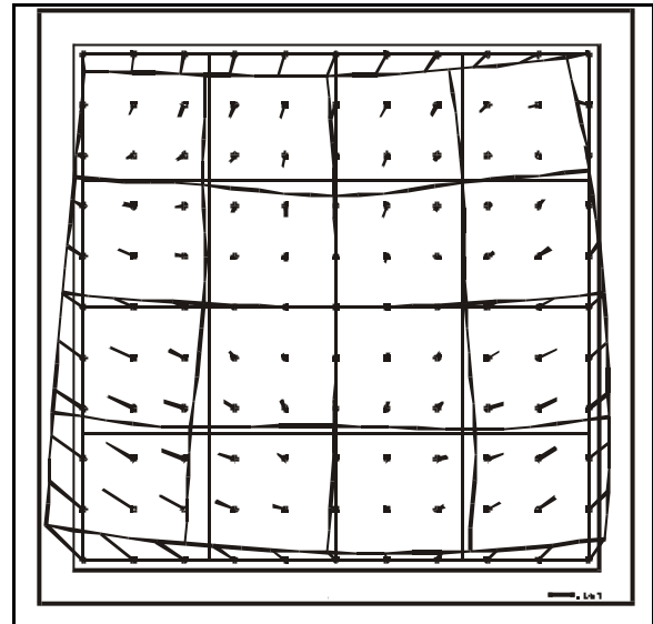
Figure 1: systematic image errors of KFA 1000, largest vector 81\mu\text{m}
