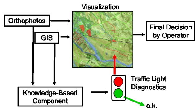
Figure 1: Workflow WiPKA-QS
