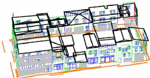
Figure 14. Combination of data from two different sources: 3D polylines of roofs based on aerial images and 3D polylines of façades from terrestrial laser scanning data
