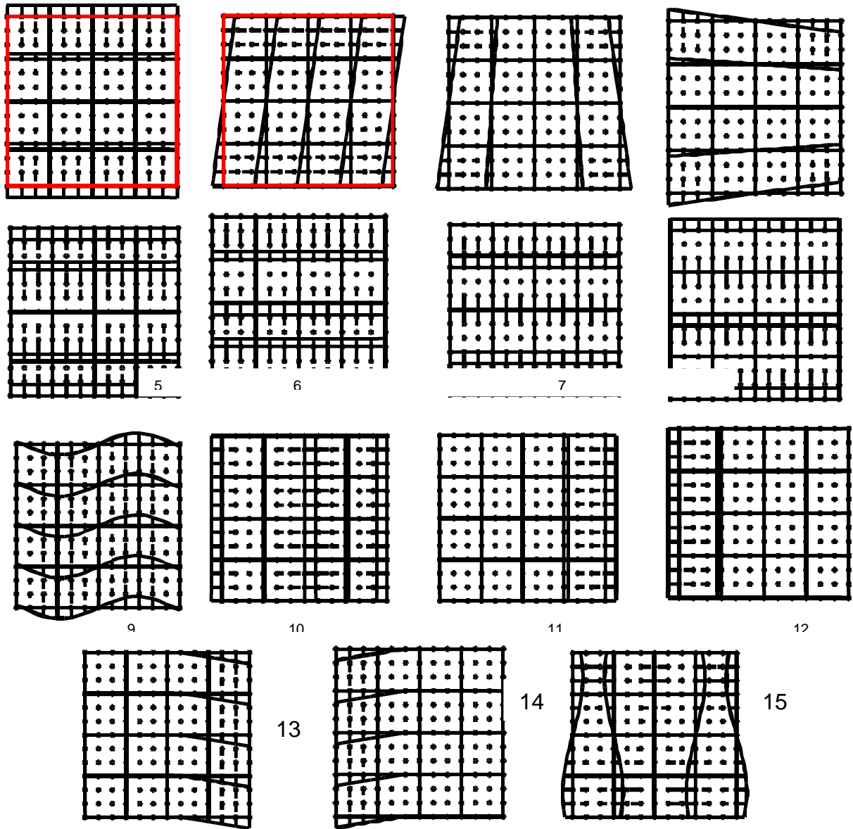
figure 11: effect of the additional parameters (BLASPO) to the image coordinates
