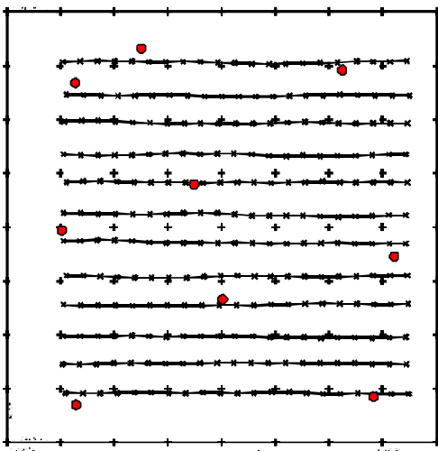
Figure 7: configuration of the check area with the control points
