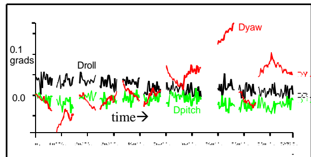
Figure 8: discrepancies of the attitude data corrected IMU – bundle block adjustment f(\text{time})
