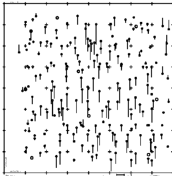
Figure 10: discrepancies at the ground coordinates Z - plot of 10% of the 1886 points
