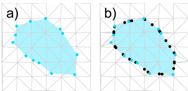
Figure 2: Integration of a DTM and an object "lake", a) original DTM TIN and object "lake", b) integrated data set
