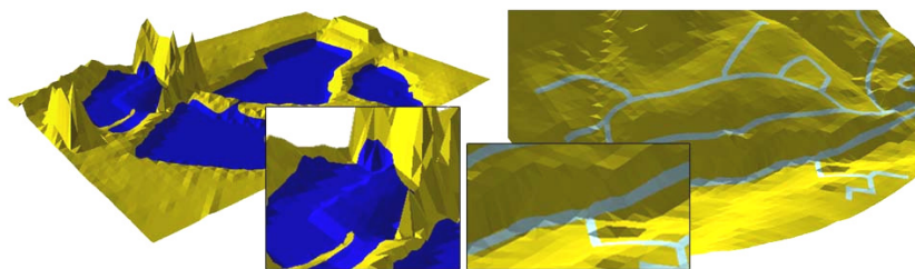
Figure 1: Results of the integration of a DTM and a 2D vector data set without considering the semantics of the topographic objects, left: lakes, right: road network
