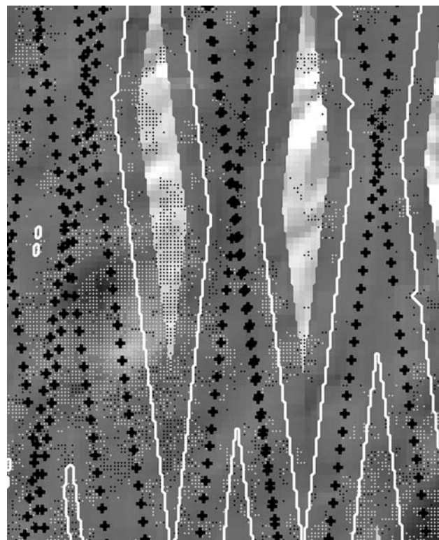
Figure 6. Intermediate result of HRSC point classification. MOLA points (black crosses) are used to define distance bands (white lines) and to derive a first DTM approximation which is used to accept HRSC points within a height tolerance band during the first iteration. The shading derived from accepted points appears smoother (dark gray area) than the not yet classified points (light gray). Accepted HRSC points are denoted in white, not (yet) accepted in black.
