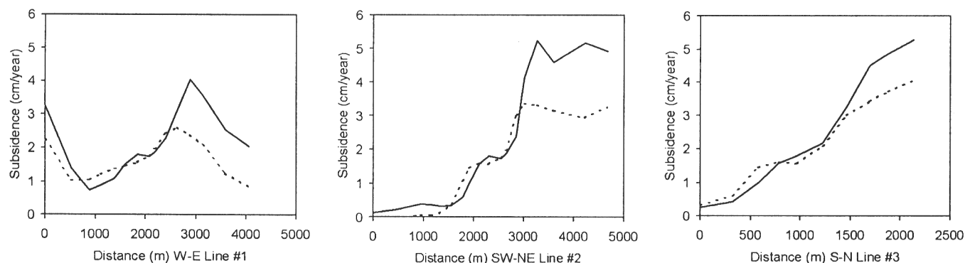
Figure 4. Profiles of the subsidence velocities determined from ERS SAR interferometry (period 1992–1993, dotted lines) and leveling surveys (period 1987–1992, normal lines) along the three leveling lines shown in Figure 3.
