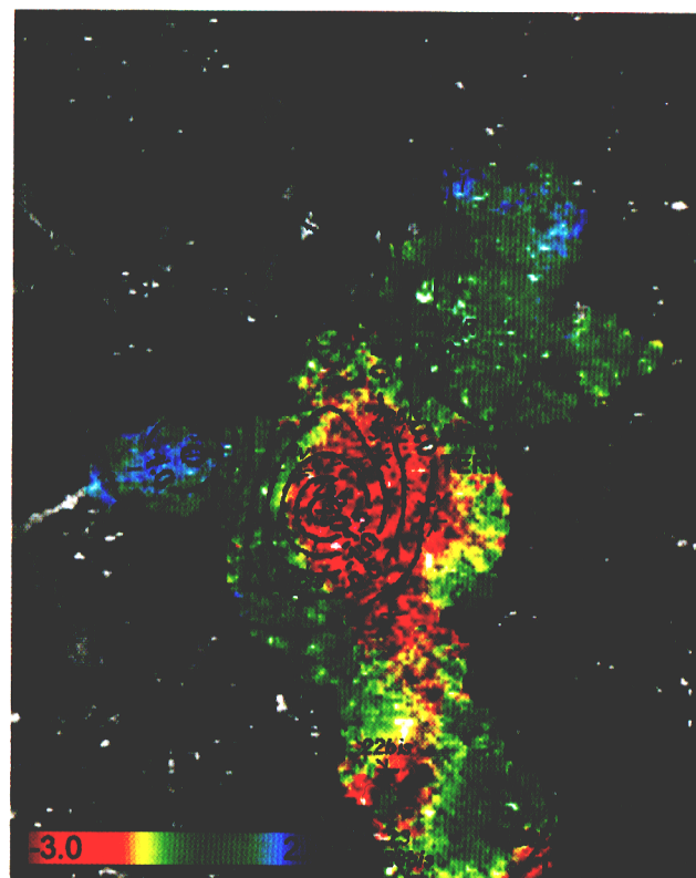
Plate 2. Map of the vertical ground movements (in mm/year) from two leveling surveys in 1991 and 1995 in the urban areas of Abano and Montegrotto Terme (data from Comune di Abano Terme and Regione del Veneto) superimposed on the ERS interferometric displacement velocity map for the time interval 1992 and 1996 (in mm/year). Also shown is the position of the benchmarks (+). The image width is about 4.5 km.
