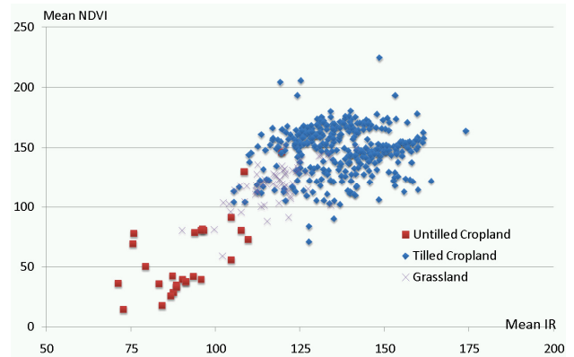
Figure 2. Scatter Plot of mean NDVI and Infrared of the objects of a reference dataset.
