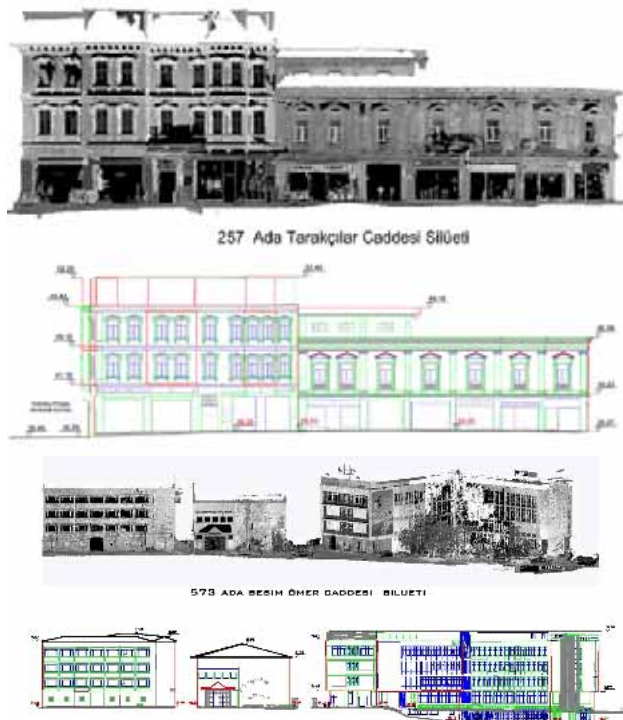
Figure 6. Detailed map of building façades using laser scanning data - laser scanning data (top) and façade plan (bottom)
