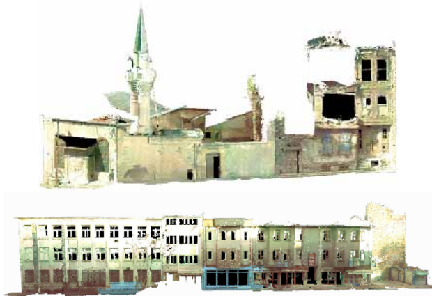
Figure 2. Coloured point cloud of building facades in the Historic Peninsula
