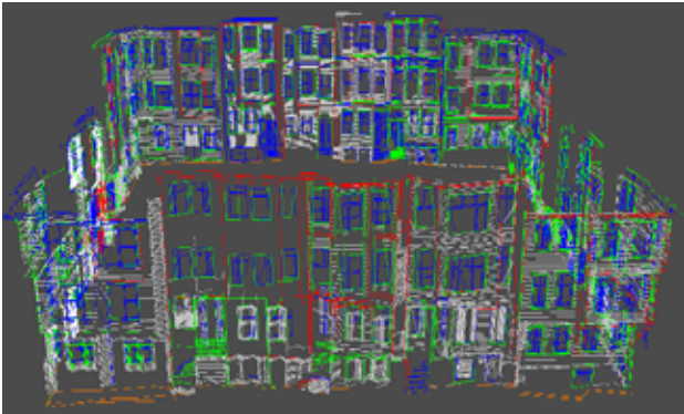
Figure 5. Mapped 3D polylines of building block façades derived from terrestrial laser scanning data
