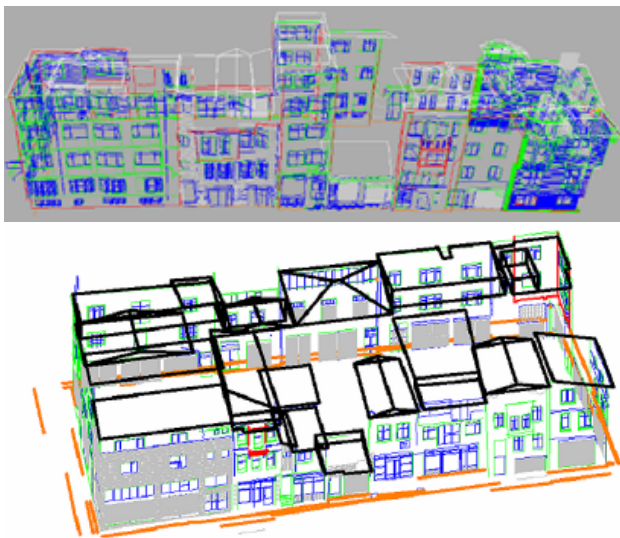
Figure 8. Combination of data from two different sources: 3D polylines of roofs based on aerial images and 3D polylines of facades from terrestrial laser scanning data
