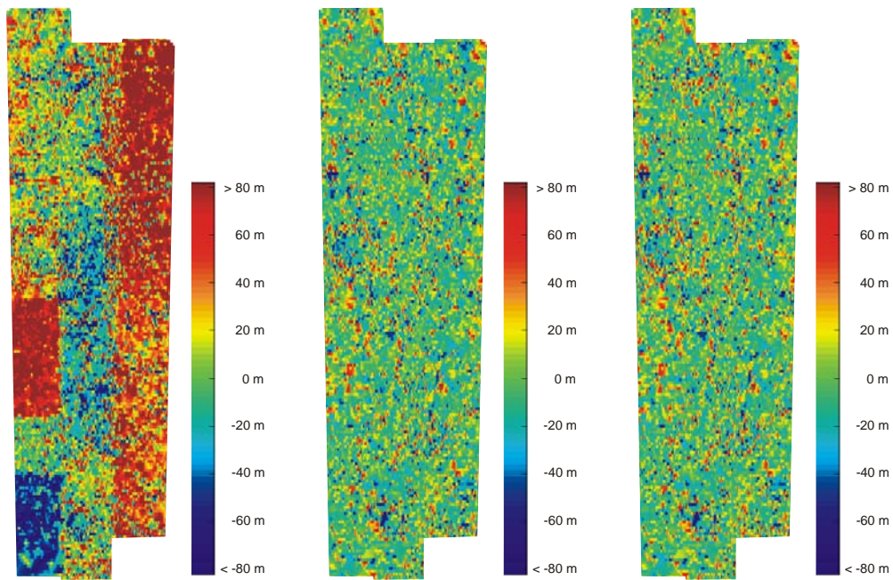
Figure 2: Differences between HRSC object points and MOLA DTM. Before (left, case A, average difference 90 m), adjusted as single strips (middle, case B, average difference 36 m), and after a full bundle adjustment within a block (right, case C, average difference 35 m).
