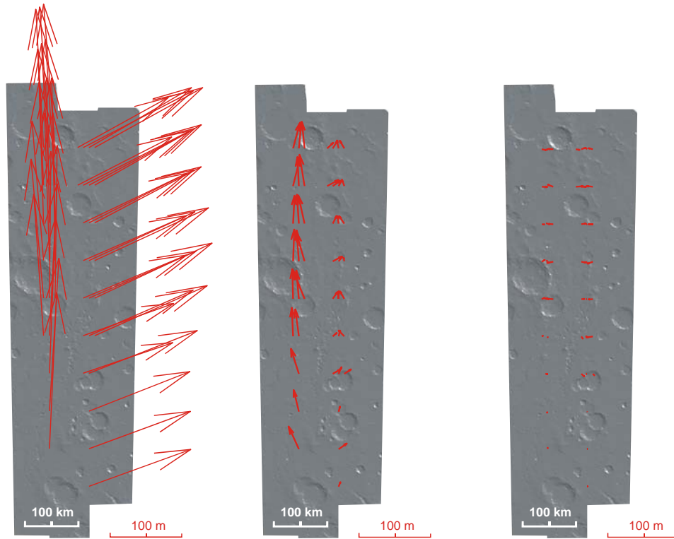
Figure 1: Average displacements between strips in planimetry. Before (left, case A), adjusted as single strips (middle, case B), and after a full bundle adjustment within a block (right, case C). Scale for right bar refers to the length of the arrows.
